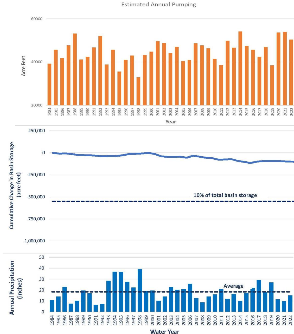
Figure 2.2.4: Estimated Annual Groundwater Pumping and Cumulative Change in Groundwater Storage Vs. Precipitation
